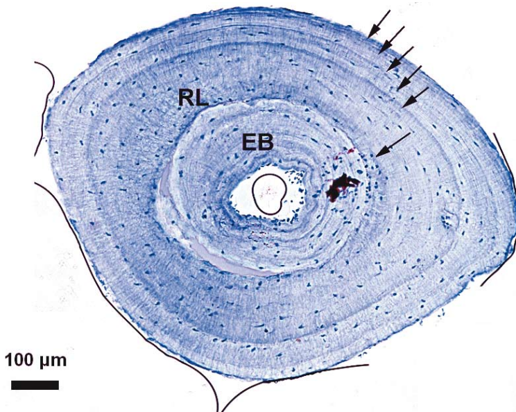
Fig. 1. Phalangeal cross-section ( \times 10 ), at the diaphyseal level, of Dyscophus antongilii from Lampirano. Female, 817 mm SVL, showing 6 LAGs (arrows), the third of which very faint. EB = endosteal bone; RL = reversal line.
