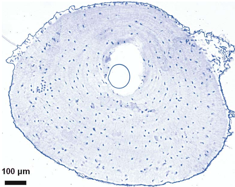
Fig. 2. Phalangeal cross-section ( \times 10 ), at the diaphyseal level, of Dyscophus antongilii from Maroantsetra. Female, 865 mm SVL, showing no LAGs, and with evident lamellar structure. ( \times 10 ).
